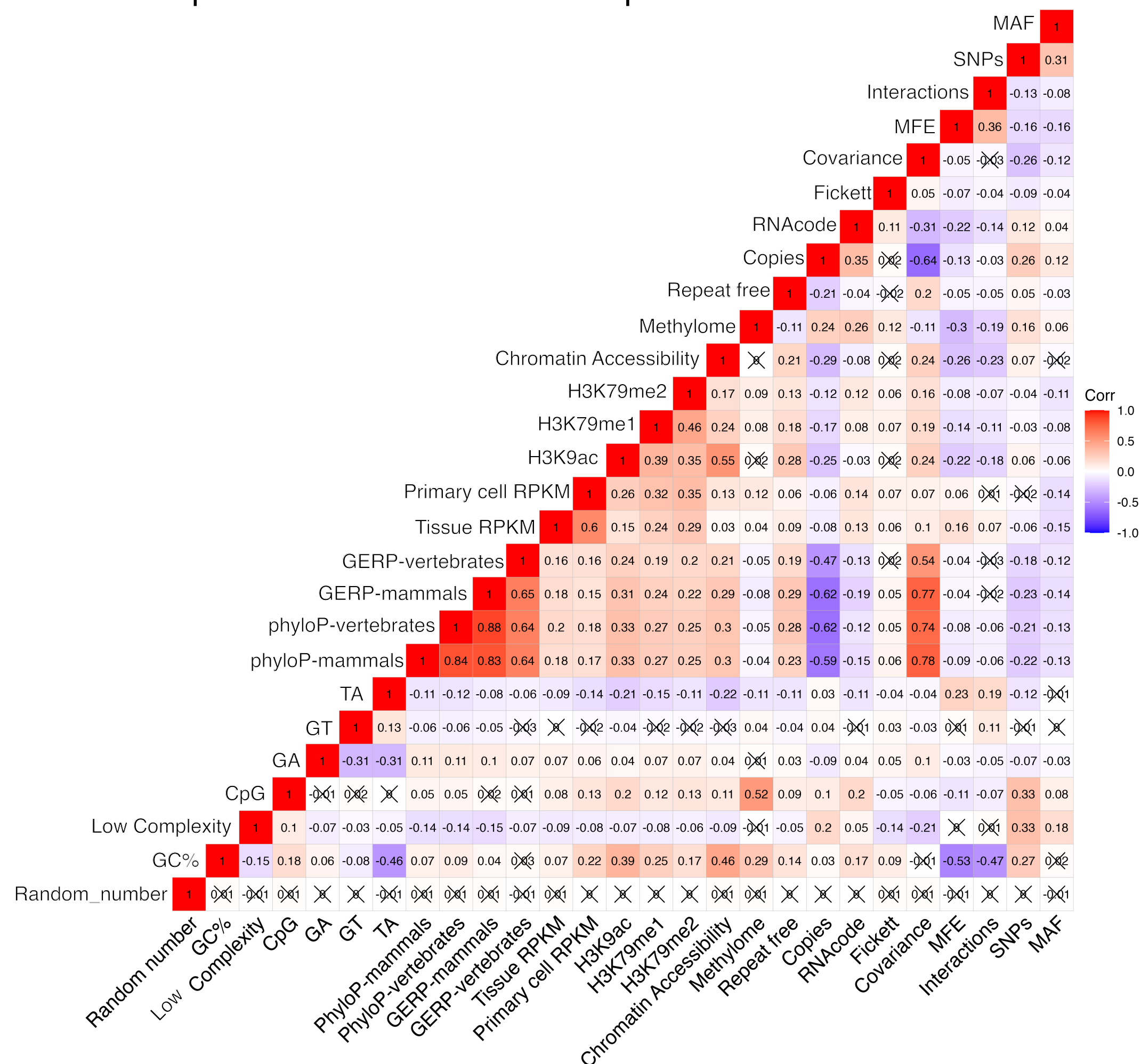
Supplementary Figure S1. mRNA correlation matrix. Spearman correlation of functionality predictors for protein-coding sequences. Positively correlated features are displayed in red and negatively correlated features in blue. Spearman’s Rho was used to determine the significance of each correlation, which were corrected for multiple testing using a Bonferroni correction. Non-significant correlations with a p-value > 0.05 have been marked with a cross.
